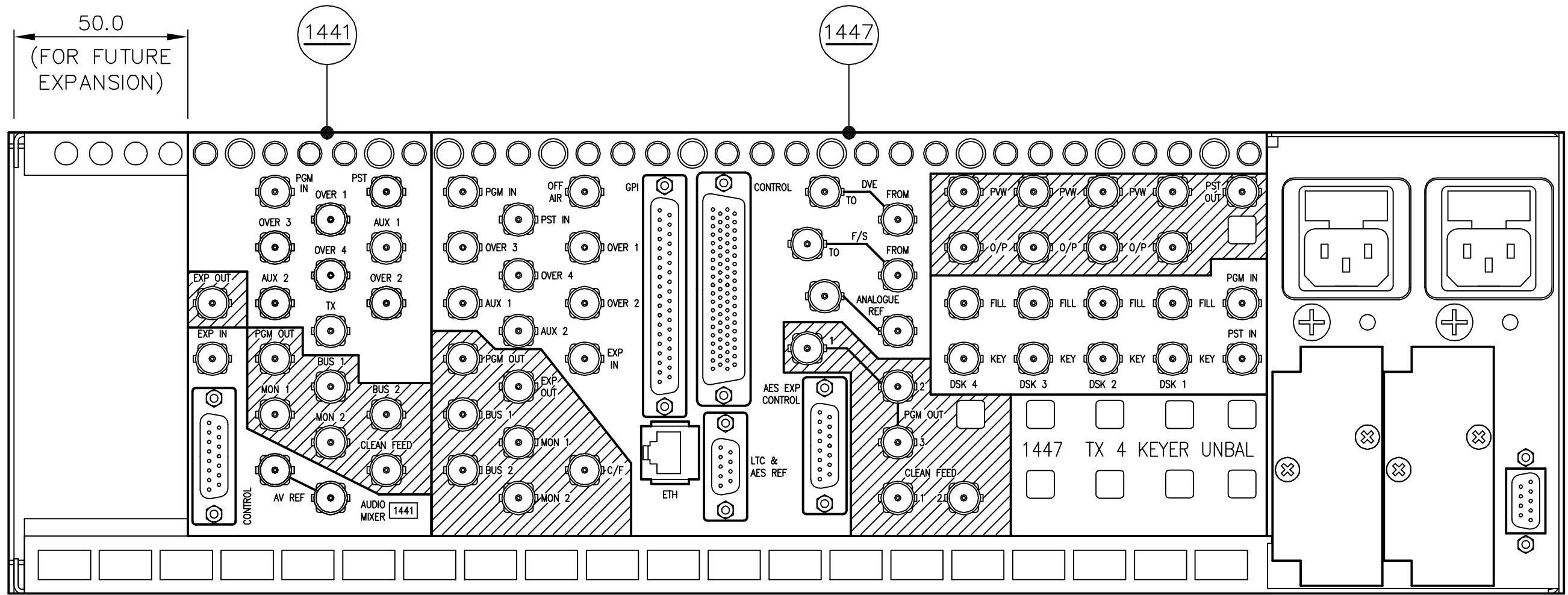
MASTER CONTROL – UNBALANCED 2 LEVEL AUDIO, 4 KEYER SYSTEM.
