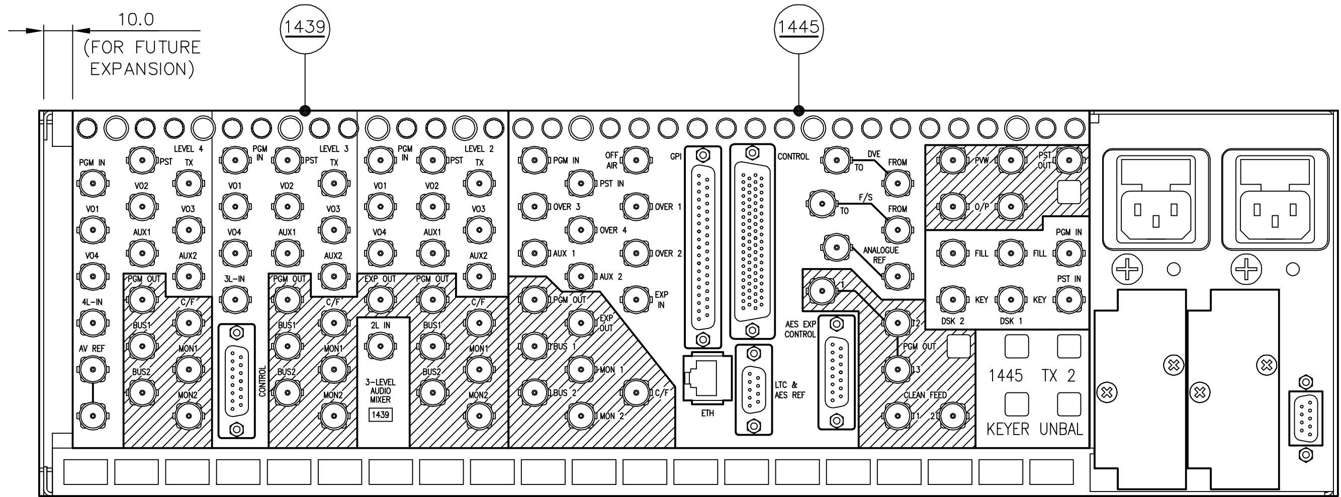
MASTER CONTROL – UNBALANCED 4 LEVEL AUDIO, 2 KEYER SYSTEM.
